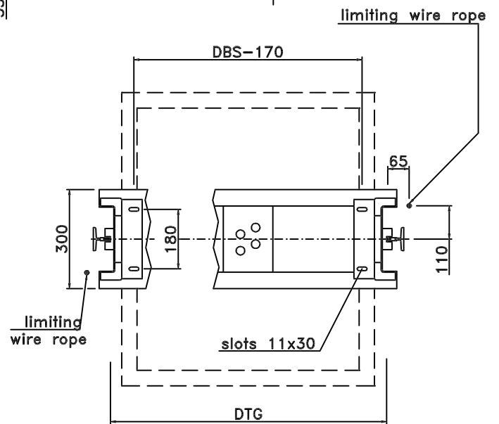
car top fixing
