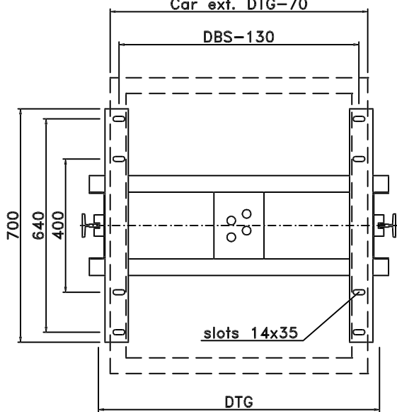
car lower fixing
